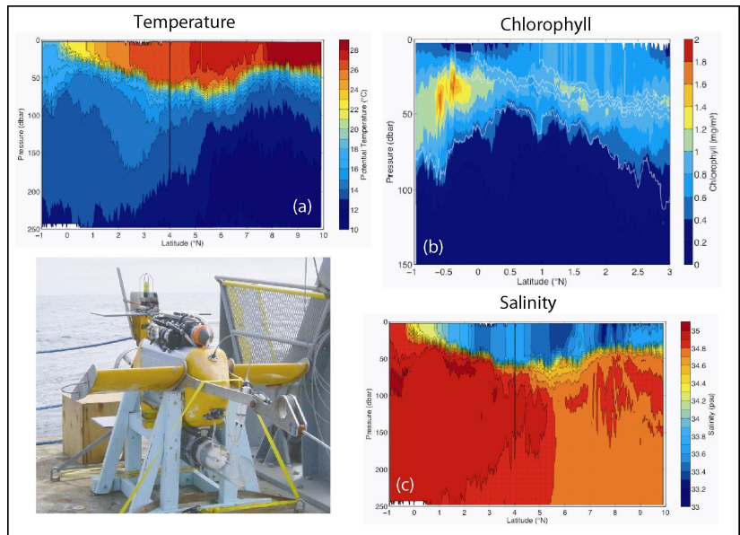
Figure 5: SeaSoar (bottom left) and examples of observational datasets collected during EPIC 2001 (photograph and figures courtesy of Jack Barth and Hemantha Wijesekera)
